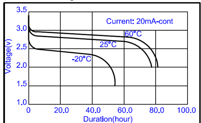
Discharge Characteristics
